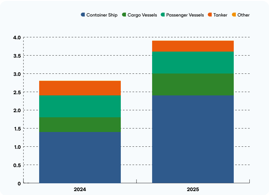
LNG BUNKERING VOL. BY RECEIVING VESSEL TYPE (IN MT)
