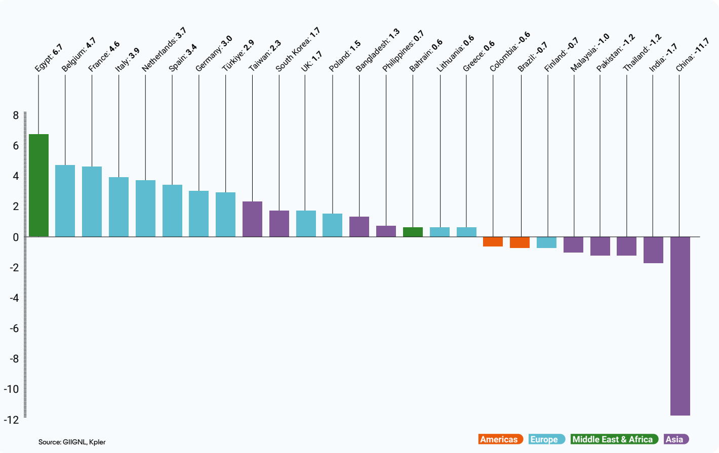
MAIN VARIATIONS IN LNG IMPORTS: 2025 VS. 2024 (MT)
