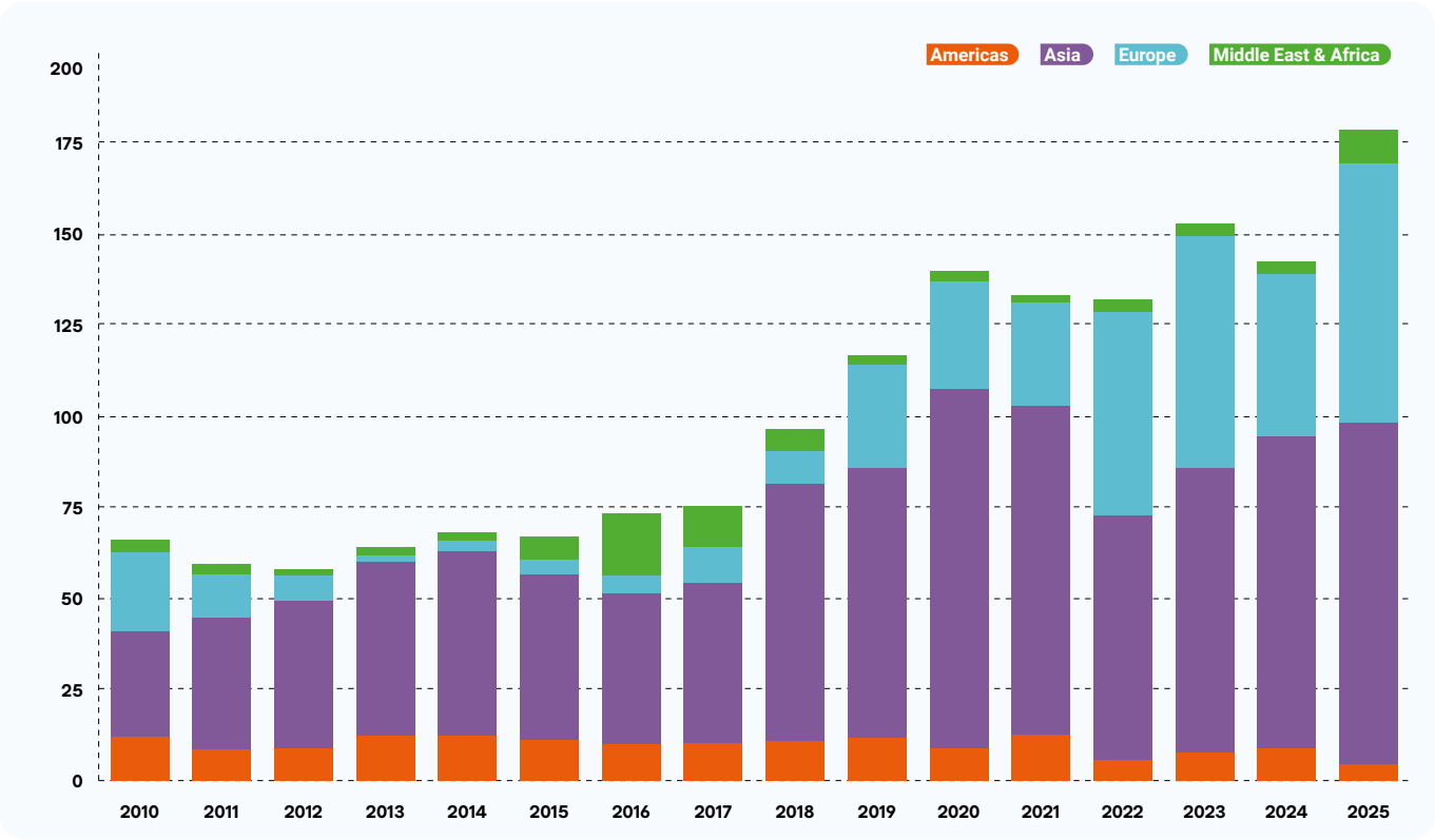
SPOT & SHORT TERM FLOWS BY IMPORTING REGION (MTPA)
